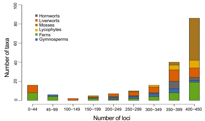
FIGURE 1. Distribution of the number of successfully sequenced loci (out of a possible 451) per taxon sample. Each locus is a relatively conserved exon from a single-copy or low-copy nuclear gene.
